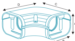
Elbow Bend 90°
